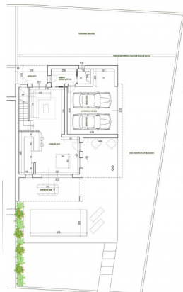
PIANO TERRA 1:100
